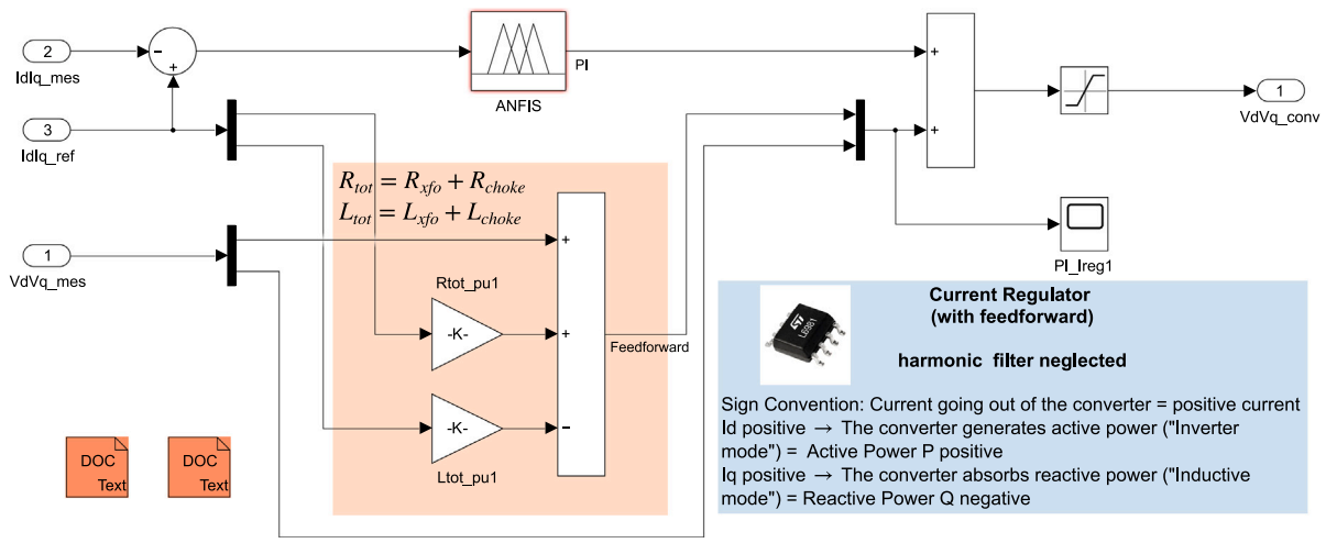
(a) A model’s subsystem, featuring several comment types: DocBlocks (on the left in apricot) and Annotations (in champagne and light blue). The Annotation in champagne color highlights a specific area of the view, while the Annotation in light blue gives general information and shows a picture. Note the formatting opportunities, including \LaTeX , in Annotations.
